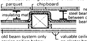
④ Insertion of new steel beam floor
